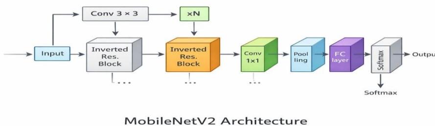
MobileNetV2 Architecture
